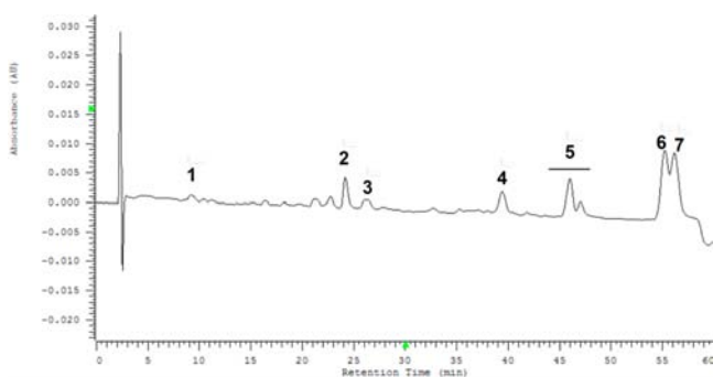
Figure 9. HPLC chromatogram (at 470 nm) of carotenoid composition of the tomato seed oil sample: (1) lutein, (2) (all- E )- \beta -carotene, (3) (9 Z )- \beta -carotene, (4) (13 Z )- + (15 Z )-lycopene, (5) (5 Z ,9' Z )- + (9 Z )- + (5 Z ,9 Z )-lycopene, (6) (all- E )-lycopene, (7) (5 Z )-lycopene. HPLC system by Merck-Hitachi; C30-column, preceded by a C18-precolum. Mobile phase: gradient of MeOH (A) and MTBE (B). T = 10 \pm 1 ^\circ\text{C} .
